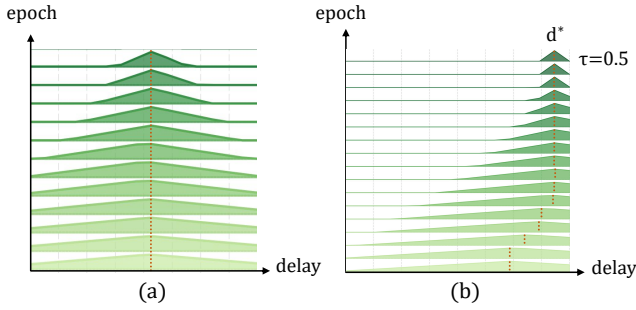
Figure 4. Visualization of delay optimization strategy. (a) Progressive sharpening of the distribution as temperature \tau anneals across training epochs. (b) Joint optimization of distribution sharpness and the learnable delay center d^* .
