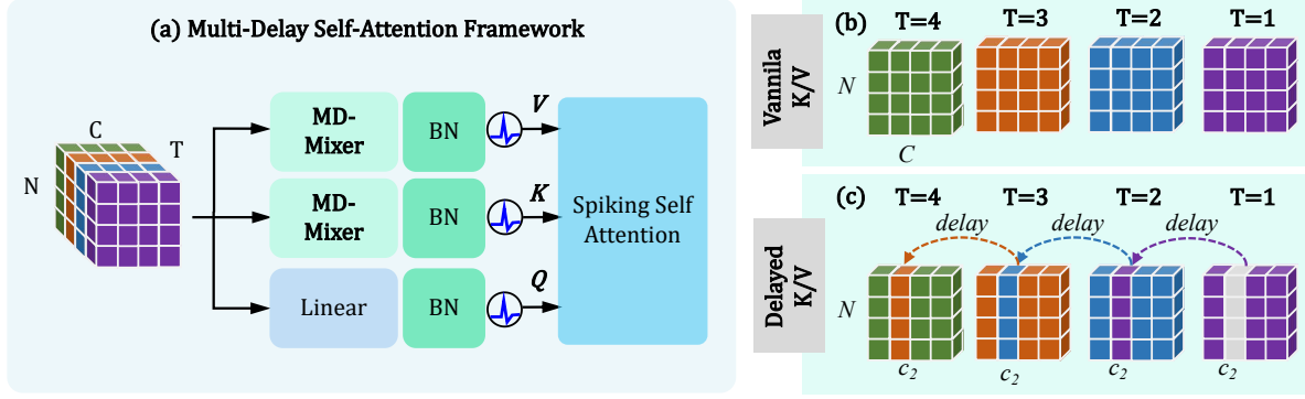
Figure 3. Illustration of the multi-delay self-attention framework. (a) The framework employs two MD-Mixer modules to generate keys (K) and values (V), and a linear projection for queries (Q), followed by batch normalization (BN) and spiking self-attention. (b) Keys and values of vanilla self-attention across timesteps (T=1 to T=4). (c) The delayed keys and values capture multi-scale temporal dependencies by aggregating historical information at learnable temporal delays.
