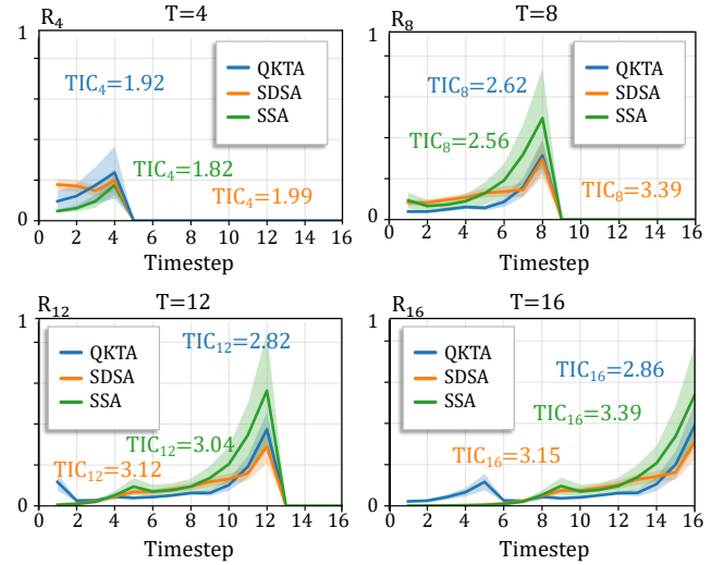
Figure 5. Visualization of reliance vectors for SSA, QKTA, and SDSA attention mechanisms integrated with MD-Mixer, based on the CIFAR10-DVS dataset.
