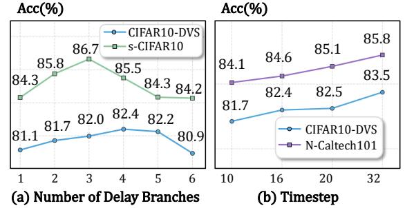
Figure 6. Impact of hyperparameters. (a) Number of delay branches on CIFAR10-DVS and s-CIFAR10. (b) Number of timesteps on CIFAR10-DVS and N-Caltech101.
