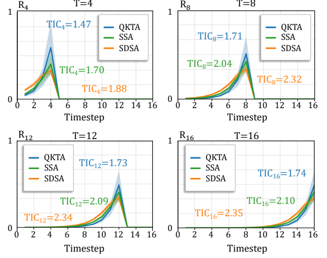
Figure 1. Visualization of reliance vectors for SSA, QKTA, and SDSA attention mechanisms, based on the CIFAR10-DVS dataset.
