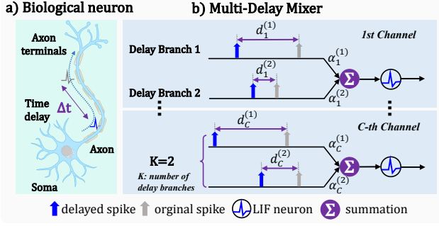
Figure 2. The proposed MD-Mixer inspired by axonal transmission delays. a) Biological inspiration. b) MD-Mixer with multiple delay branches and channel-wise aggregation, where K = 2 is shown for illustration.
